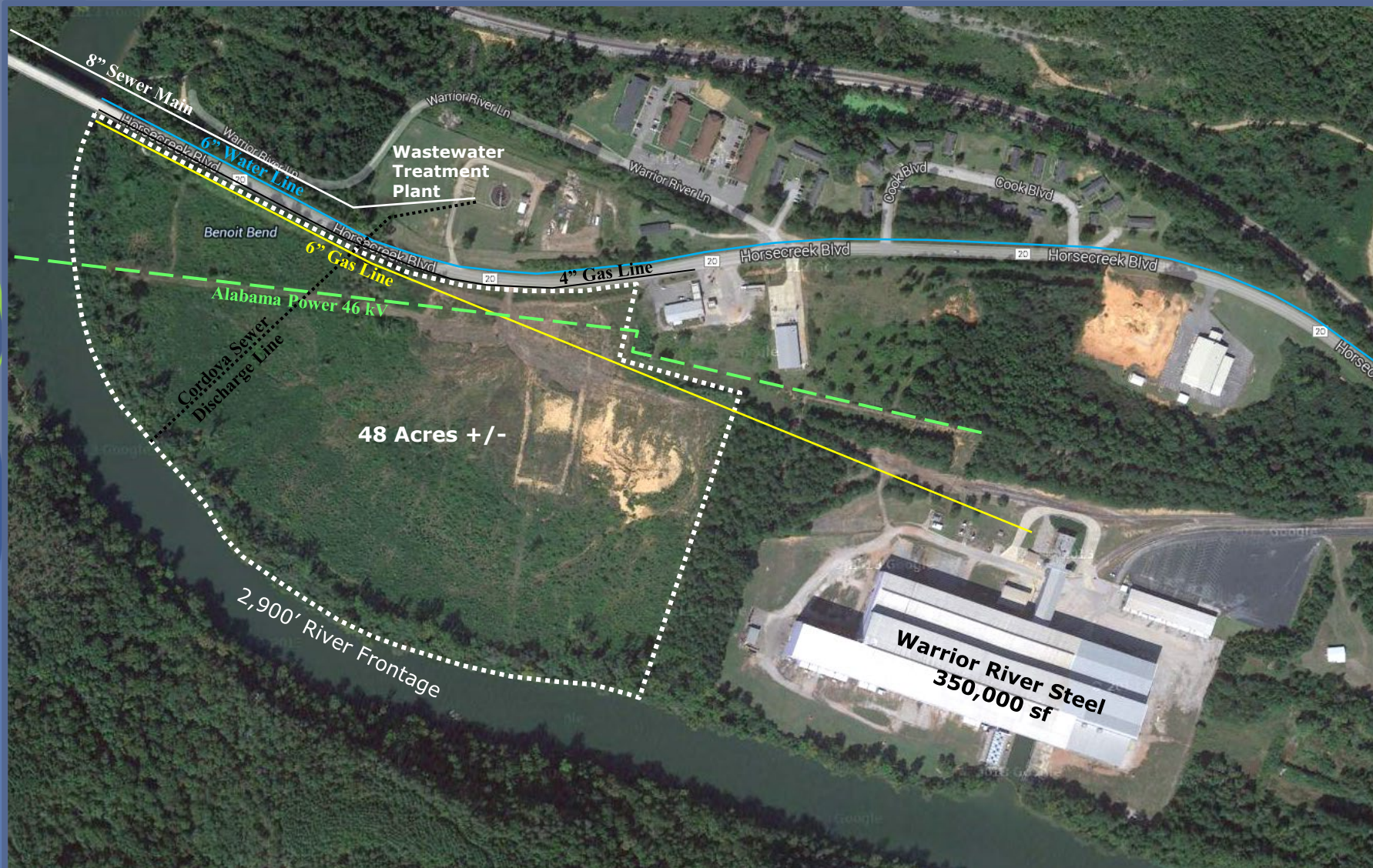
Cordova River Site – Utilities Map
